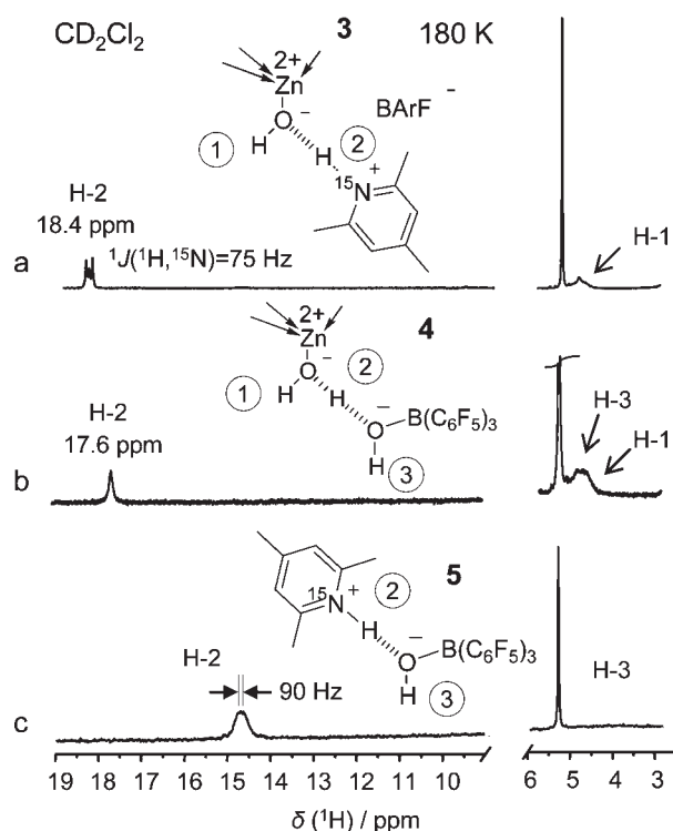
Figure 2. Partial 1 H NMR spectra at 180 K of 3 (a), 4 (b), and 5 (c) dissolved in CD 2 Cl 2 .
