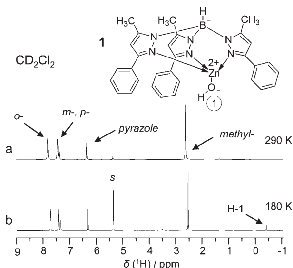
Figure 1. 1 H NMR spectra of [Tp Ph,Me ZnOH] dissolved in CD 2 Cl 2 at 290 K (a) and 180 K (b). S denotes the solvent.
